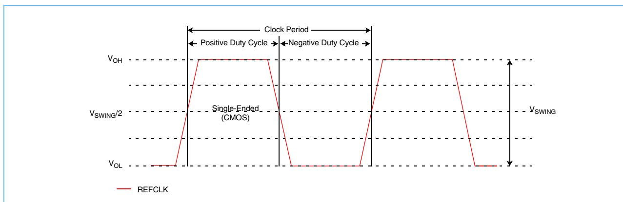
Figure 6-8. Single-Ended Processor Reference Clocks (Period and Duty-Cycle Measurement Points)
