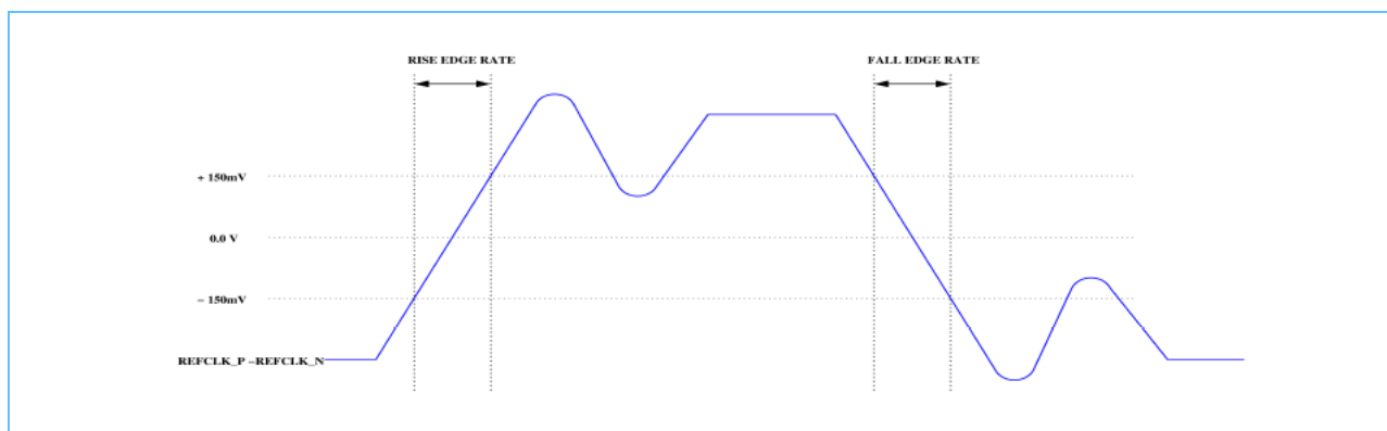
Figure 6-5. Differential Measurement Points for Rise and Fall Times
